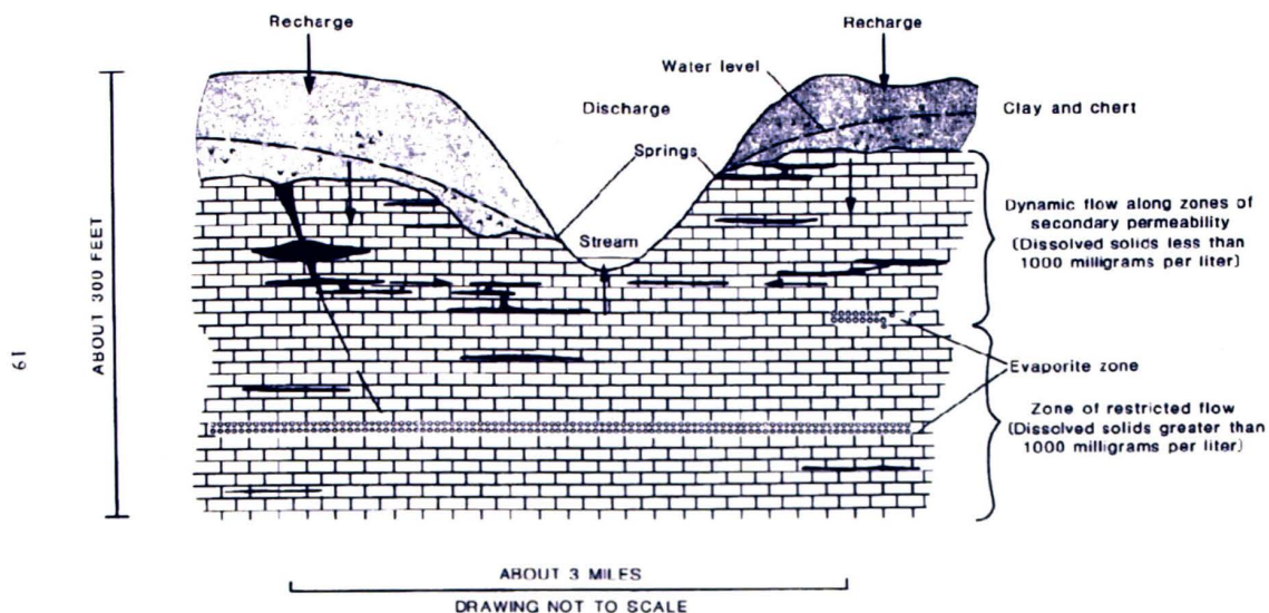
Fig. 3. Conceptual model of ground-water occurrence in the limestones of the Highland Rim aquifer system from Brahana & Bradley (1986).
